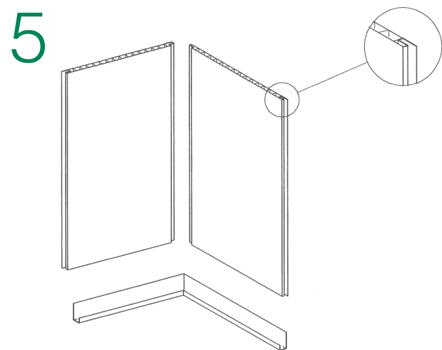
CLADDING & STARTER TRIM — FIG.5
