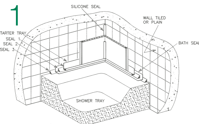
INTERNAL CORNERS - BASE DETAIL — FIG.1
