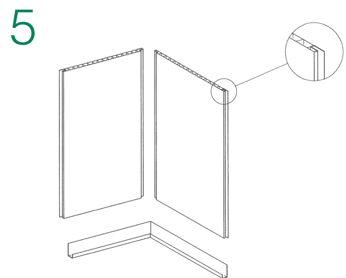
CLADDING & STARTER TRIM — FIG.5
