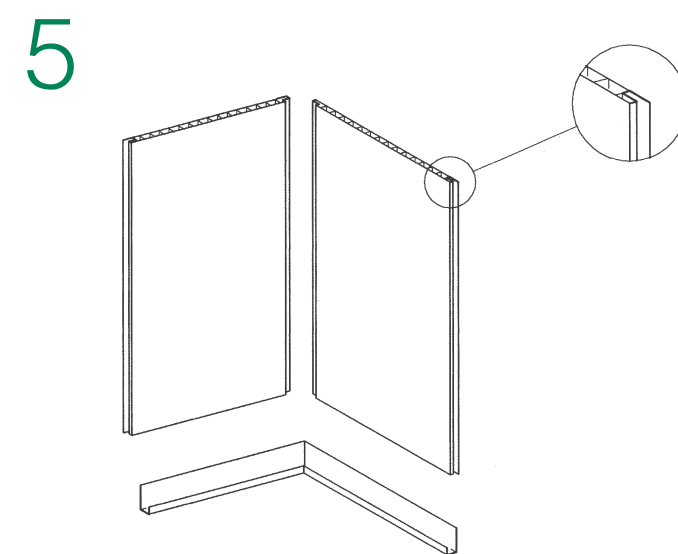
CLADDING & STARTER TRIM — FIG.5
