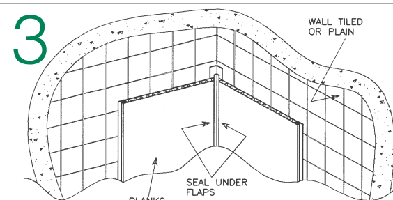
INTERNAL CORNERS (USING PVC PROFILE) — FIG.3
