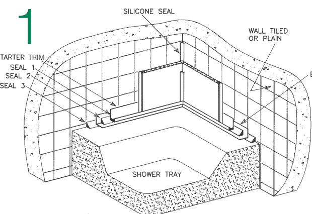
INTERNAL CORNERS - BASE DETAIL — FIG.1
