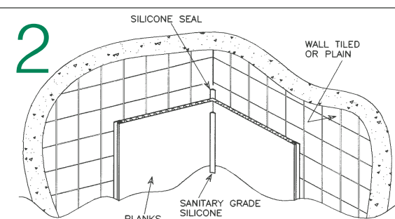
INTERNAL CORNERS (USING SEALANT) — FIG.2
